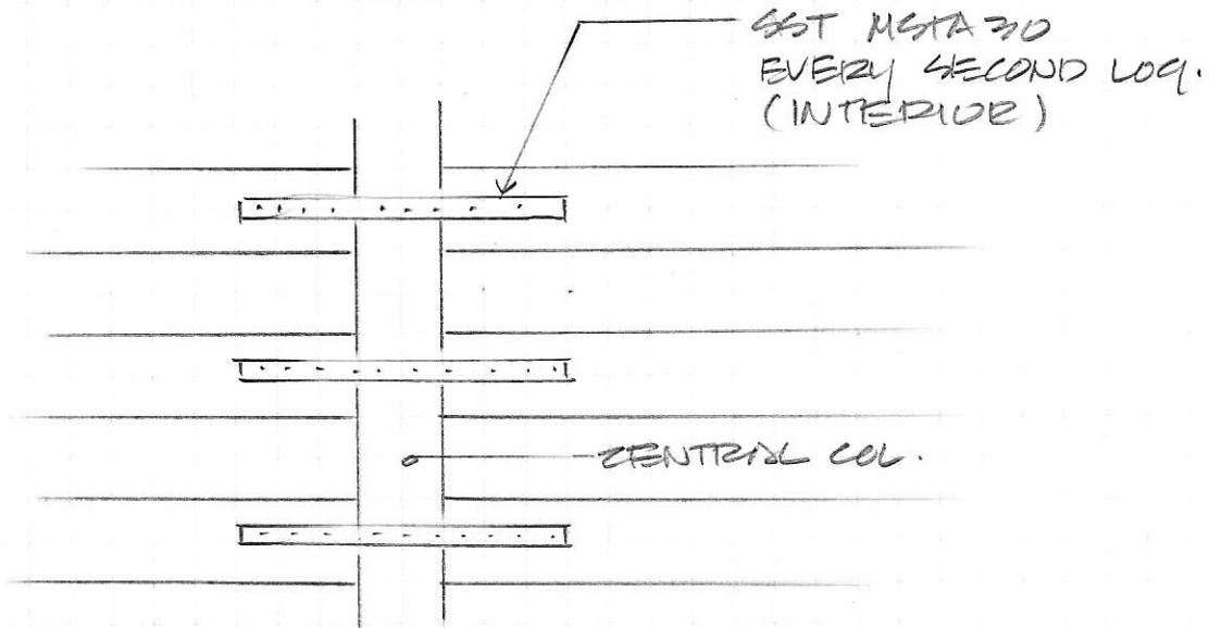
WALL TO COLUMN TIES
