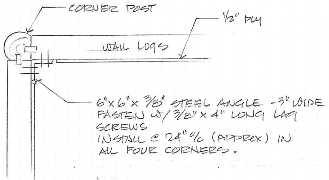
INSIDE CORNER CONNECTION
